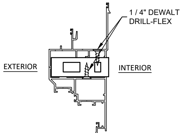
U 3 SH TO CS HORIZONTAL HEAVY MULL
