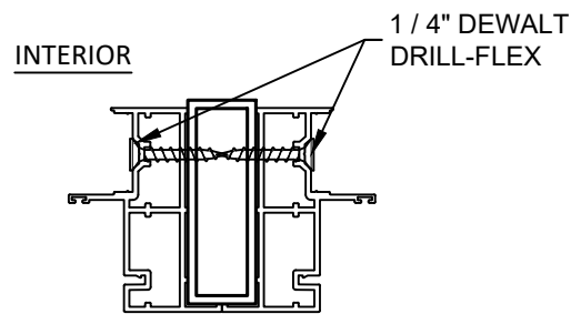
A 2 FW TO FW VERTICAL OR HORIZONTAL LIGHT MULL
