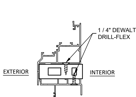
T 3 CS TO SH HORIZONTAL HEAVY MULL
