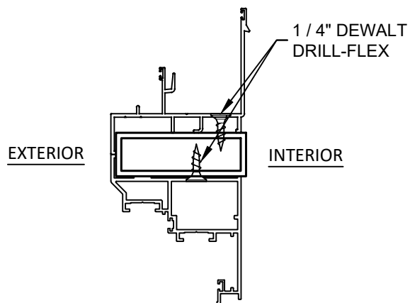
J 2 SH TO CS HORIZONTAL LIGHT MULL
