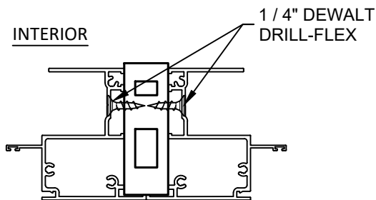
Q 3 SH TO SH VERTICAL HEAVY MULL
