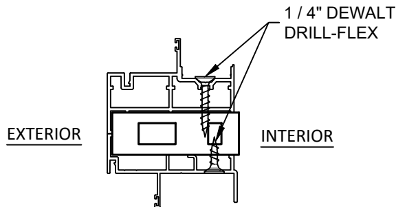
R 3 FW TO SH HORIZONTAL HEAVY MULL
