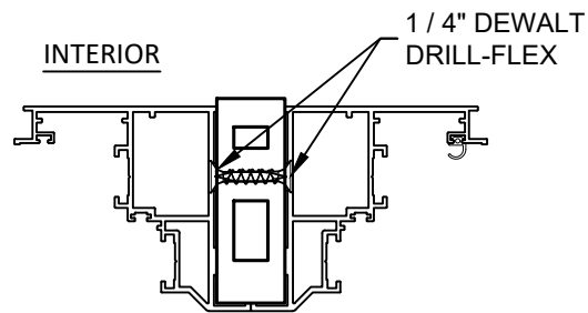
O 3 CS TO CS VERTICAL OR HORIZONTAL HEAVY MULL
