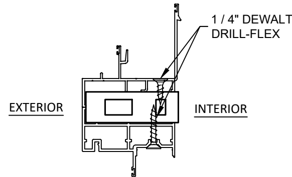
S 3 SH TO FW HORIZONTAL HEAVY MULL
