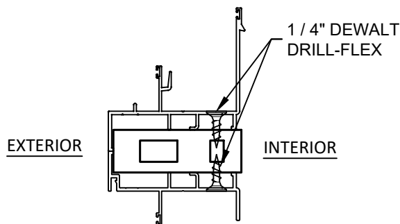
V 3 SH TO SH HORIZONTAL HEAVY MULL
