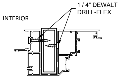
B 2 FW TO CS VERTICAL OR HORIZONTAL LIGHT MULL
