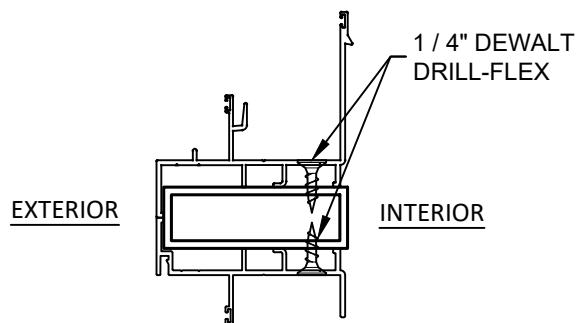
K 2 SH TO SH HORIZONTAL LIGHT MULL
